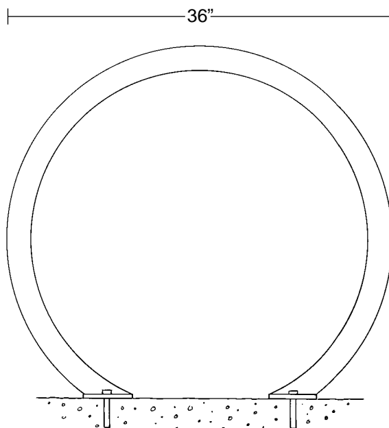
SC RACK SIDE VIEW
